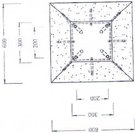
I.P. VIEW SCALE 1 : 15
